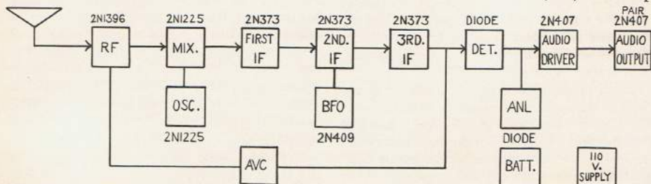
GC-1 BLOCK DIAGRAM
