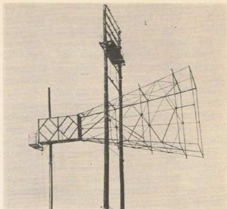
Experimental horn antenna during installation several years ago at the Muscle Shoals, Ala. CATV system. An early, and still operating, design to reject interfering signals.
