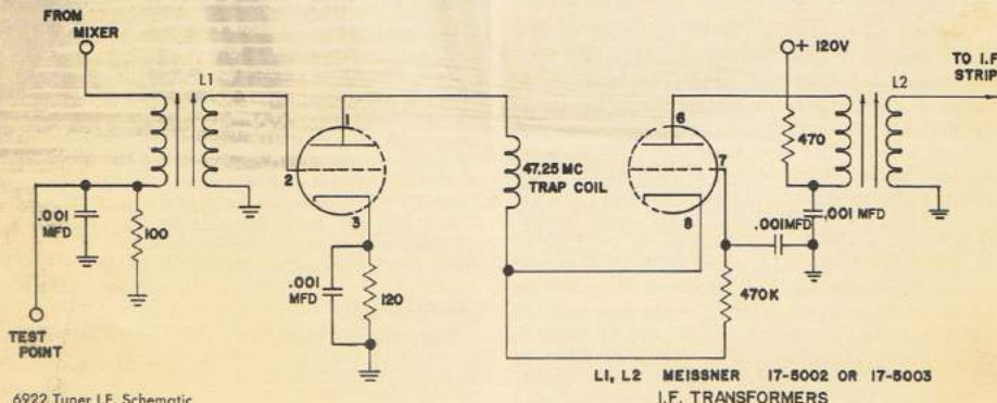
6922 Tuner I.F. Schematic
