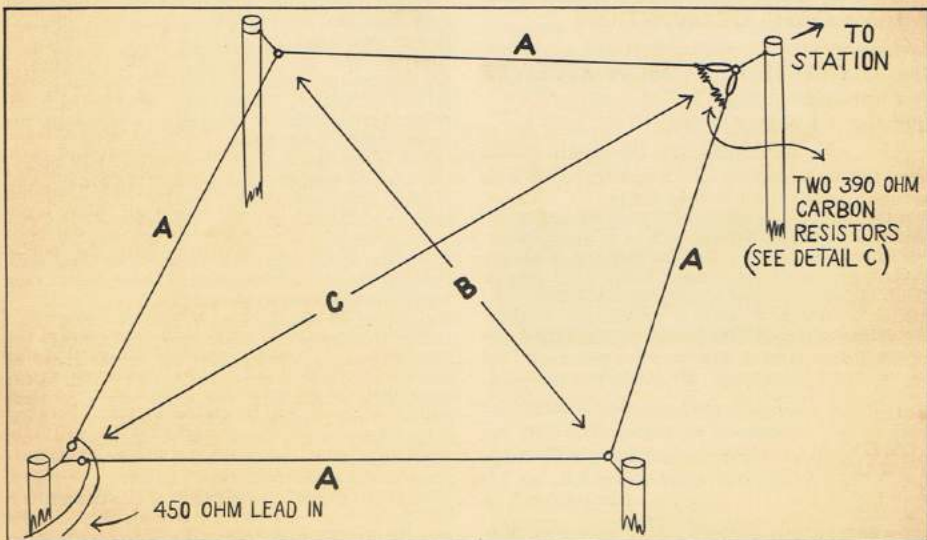
Typical One Bay Rhombic
