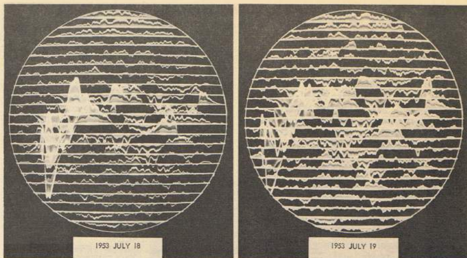
SOLAR MAGNETOGRAMS
